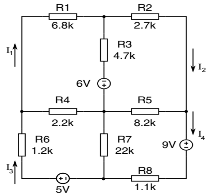
Figure 1: Example circuit, drawn from Boylestad "Introductory Circuit Analysis" 12th ed, figure 118.
