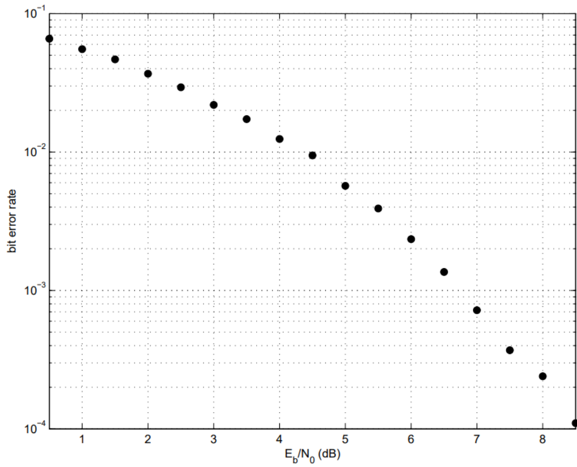
Figure 1: Typical Bit-Error-Rate Plot
