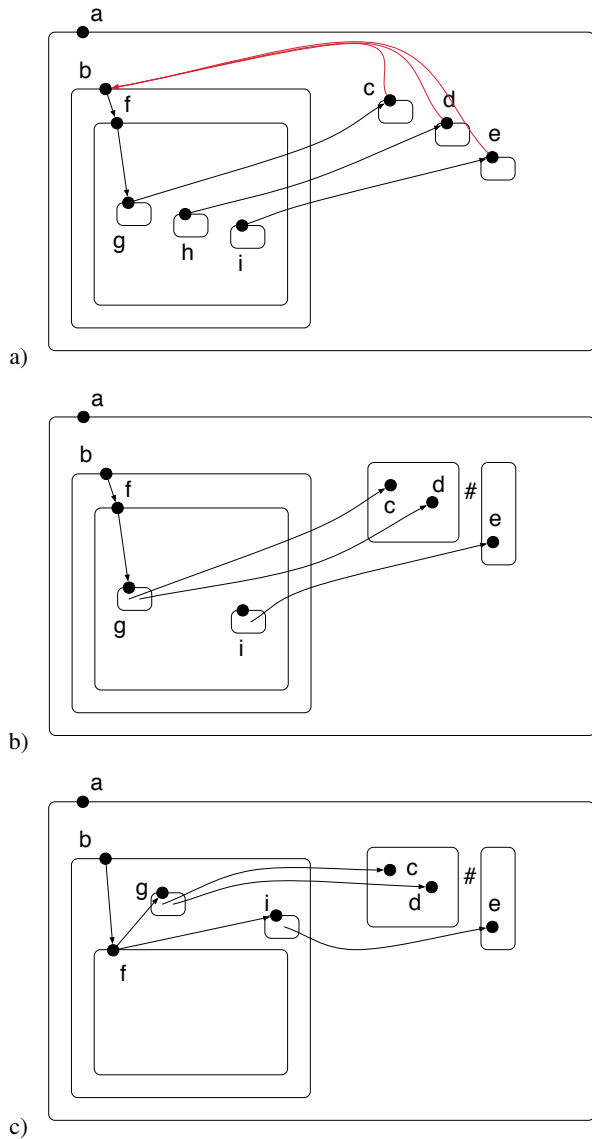
Figure 1. Ownership graphs corresponding to our three scenarios. Arrows denote references and red arrows denote absence of references.
