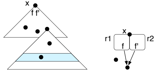
Figure 2. Joe_1 (left) and OOFX (right). In Joe_1 , each object defines a single subheap but it is possible to talk about effects on different strands of the subheap (e.g., the teal-colored stripe). In OOFX, regions are shallow and encapsulate fields only, not the contents of the fields which may be shared (with the exception of unshared fields).
