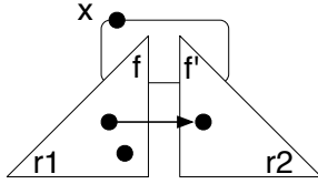
Figure 3. Regions as Owners in Joelle.
