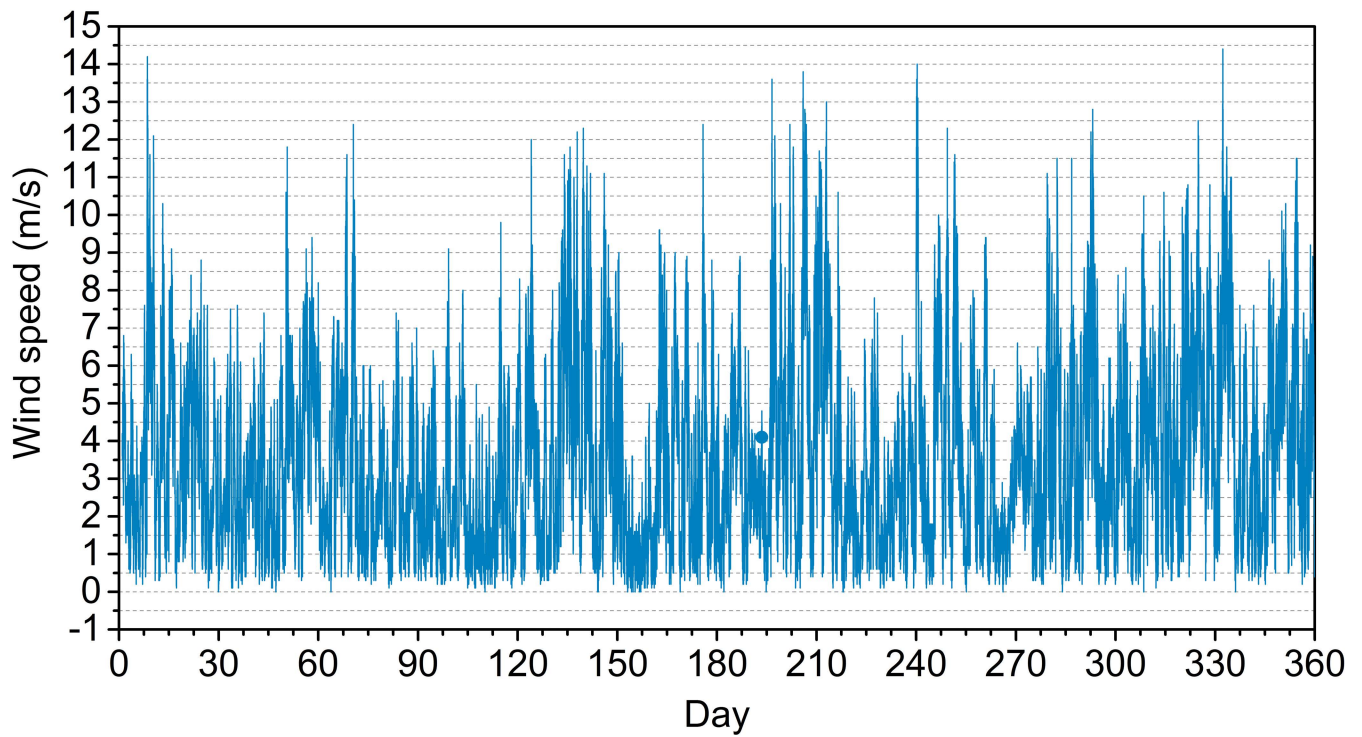
Figure 3: Wind speed vs days.
