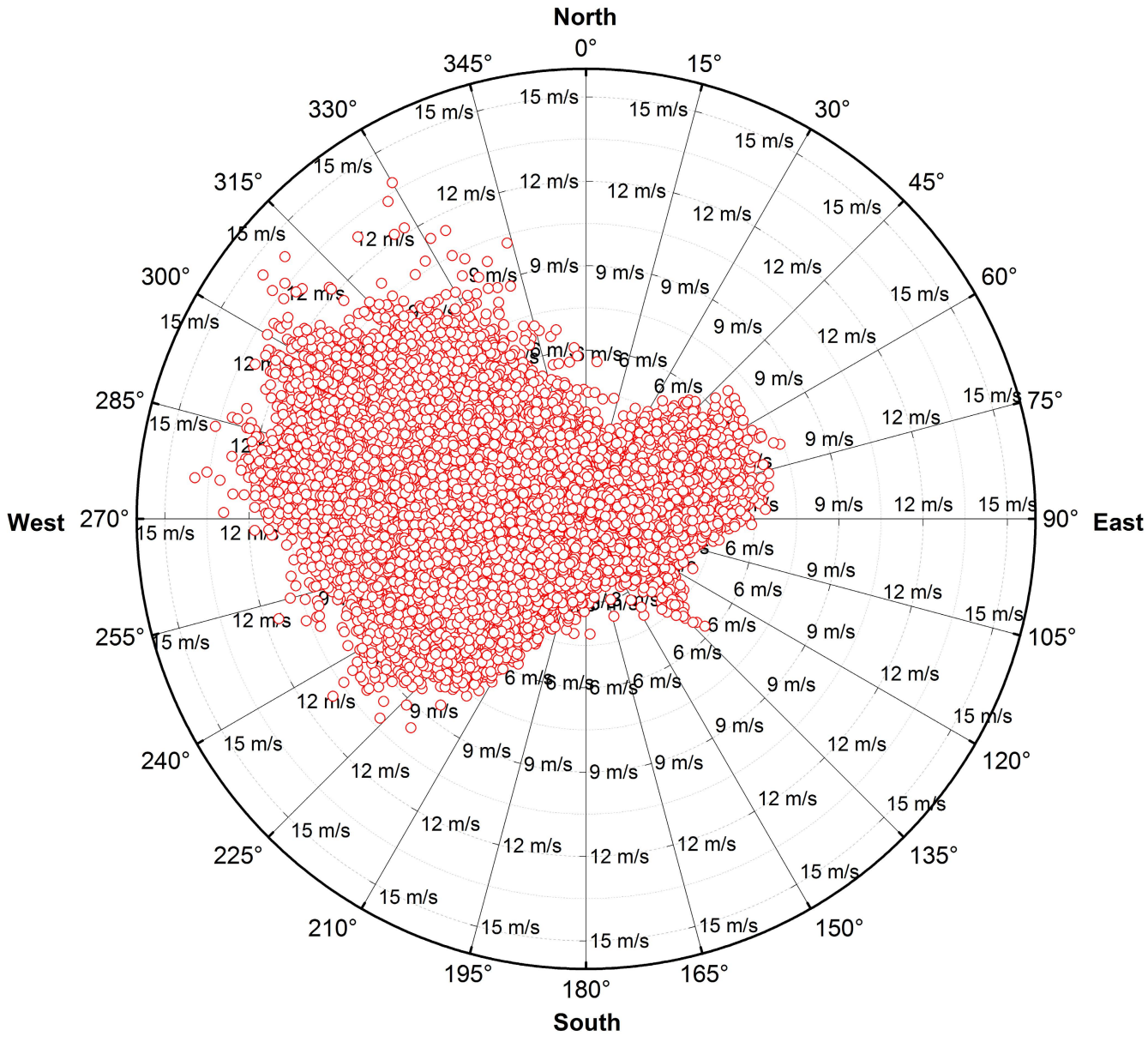
Figure 5: Wind rose diagram.
