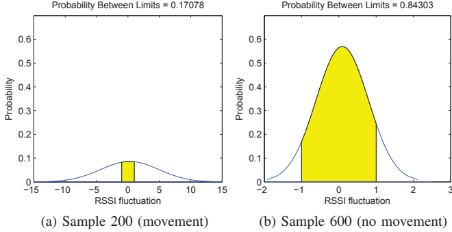
Fig. 5. Normal distribution showing probability in fluctuation range [-1,1]
