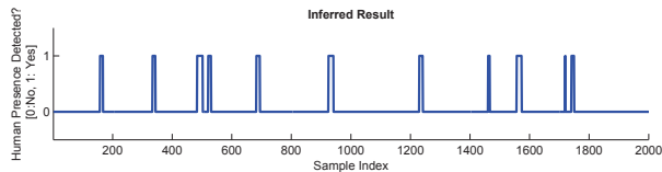
Fig. 10. Detection of pedestrian traffic along corridor
