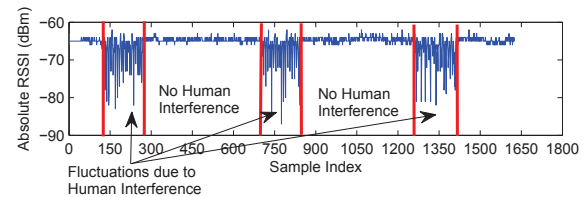
Fig. 2. Absolute RSSI reading
