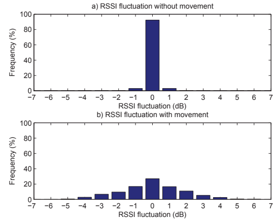
Fig. 1. RSSI Fluctuation Patterns [10]
