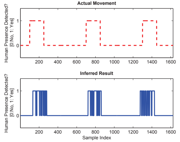
Fig. 7. Inferred presence of human movement using RSSI Fluctuations
