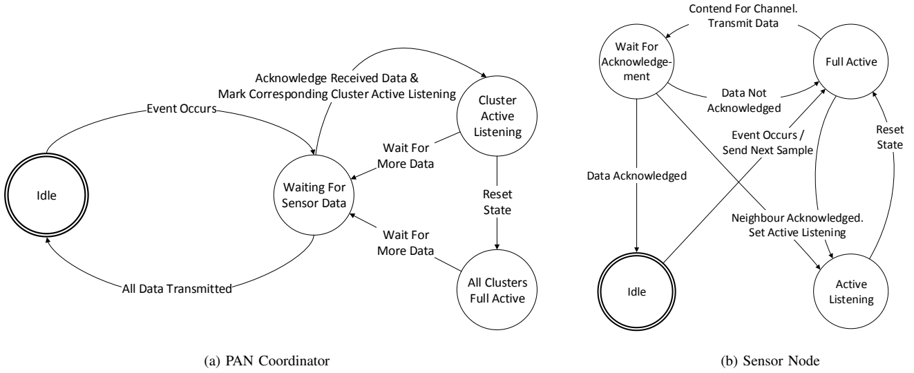
Fig. 2: State Transition Diagrams
