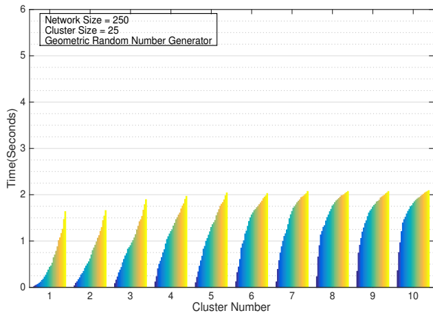
(c) IEEE802.15.4 with Geometric Random Backoff Slot Selection
