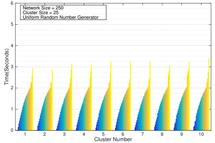
(b) Cluster-centric MAC with Uniform Random Backoff Slot Selection
