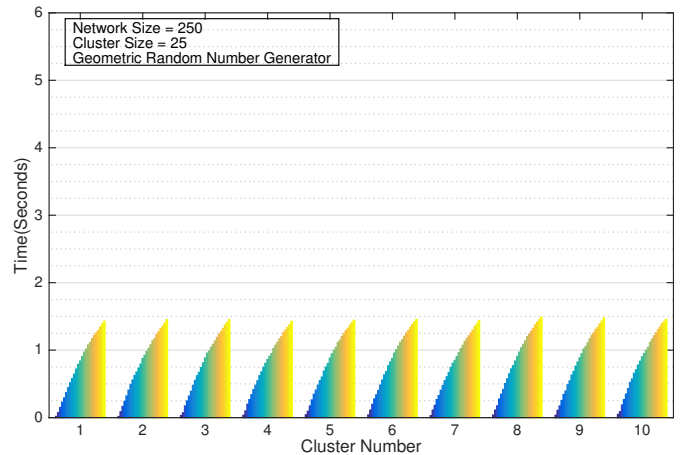
(d) Cluster-centric MAC with Geometric Random Backoff Slot Selection
