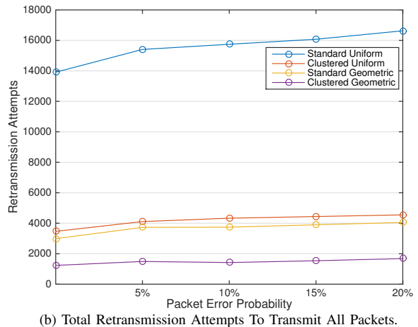
Fig. 5: Lossy Environment (N=250, C=10)
